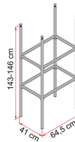
Garage System Standard
